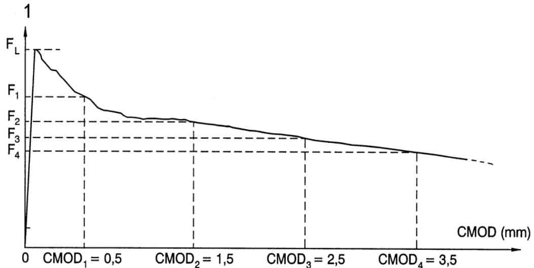
Typical Load deformation Diagram
