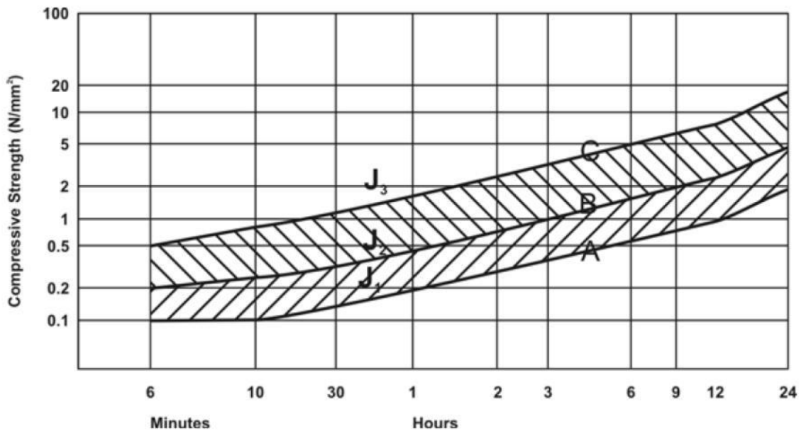
Figure 3.10.4-1: Early Strength Requirement for Shotcrete
