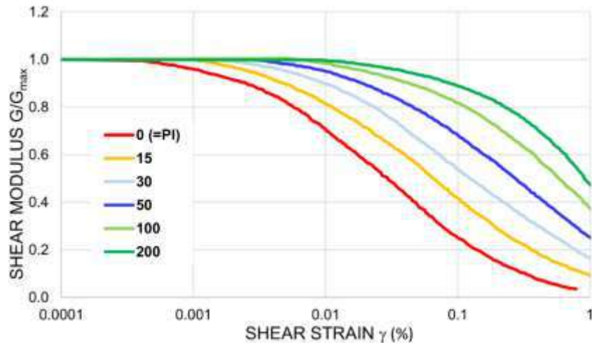
FIG. 4 TYPICAL NORMALISED SHEAR MODULUS G_D/G_{MAX} — SHEAR STRAIN \gamma CURVE OF SOIL FOR DIFFERENT VALUES OF PLASTICITY INDEX FOR ANY VALUE OF \sigma'_m
