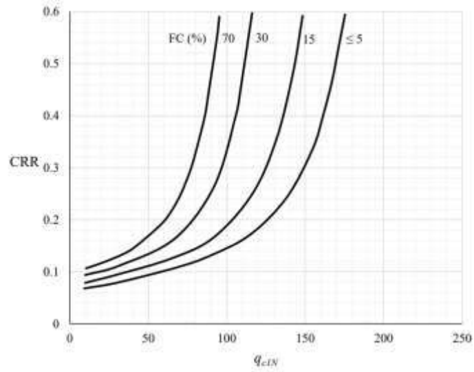
FIG. 6(A) CPT
