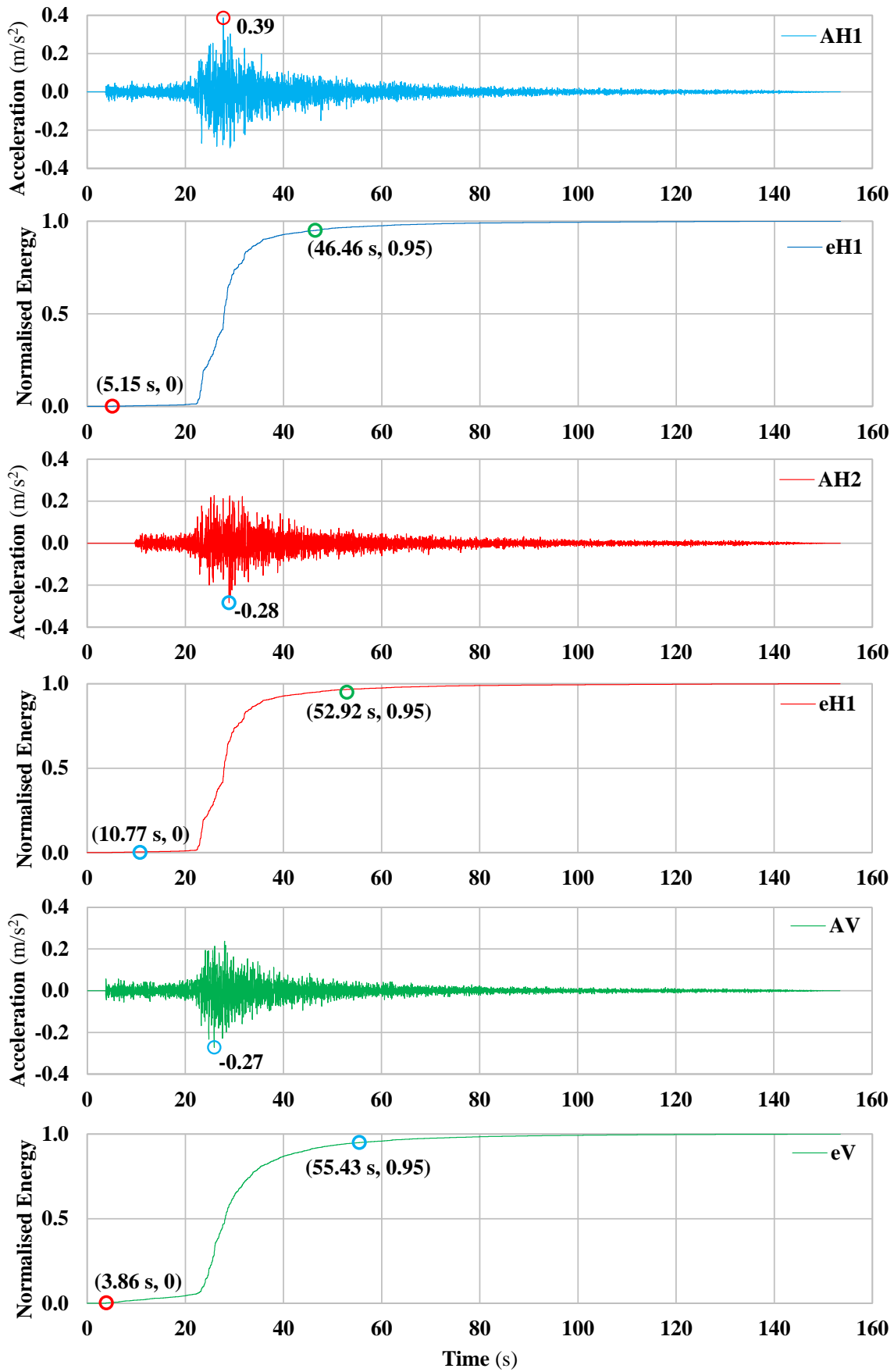
FIG. 16 GROUND MOTIONS HISTORIES SHOWING DURATION AT WHICH TO 95 PERCENT OF THE CUMULATIVE ENERGY IS INPUT TO THE STRUCTURE
