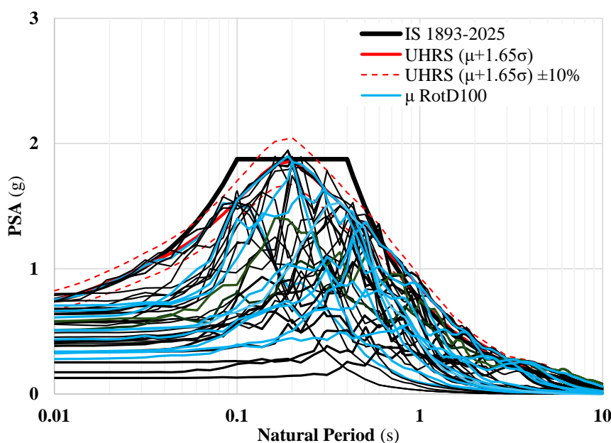
FIG. 15 30 SELECTED GROUND MOTIONS AT SITE CLASSES A AND B FOR EARTHQUAKE ZONE VI
