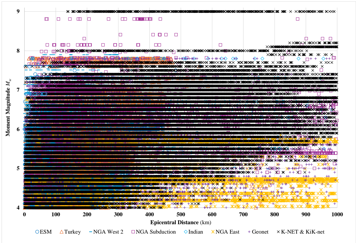
FIG. 12 DISTRIBUTION OF M_w AND R_{epi} OF THE GROUND MOTIONS CONSIDERED IN THE GROUND MOTION LIBRARY
